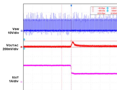
Transient Response
