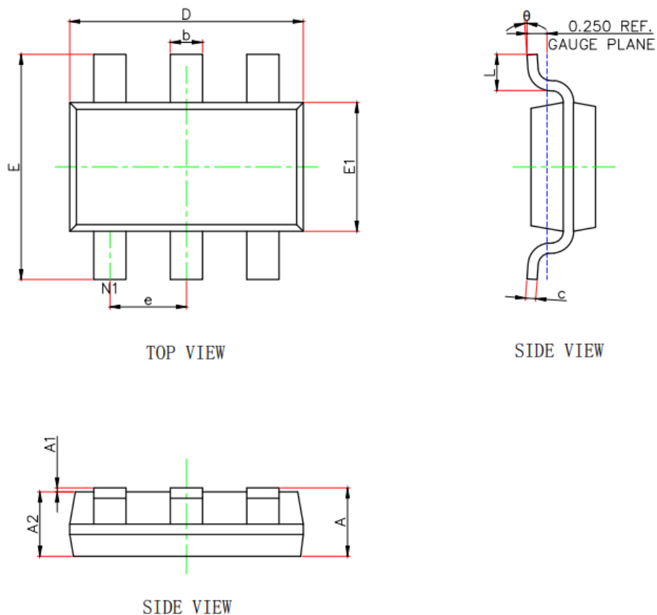
TSOT-23-6L(16R) (FC) PACKAGE OUTLINE DIMENSIONS
