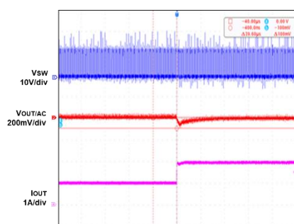
Transient Response
